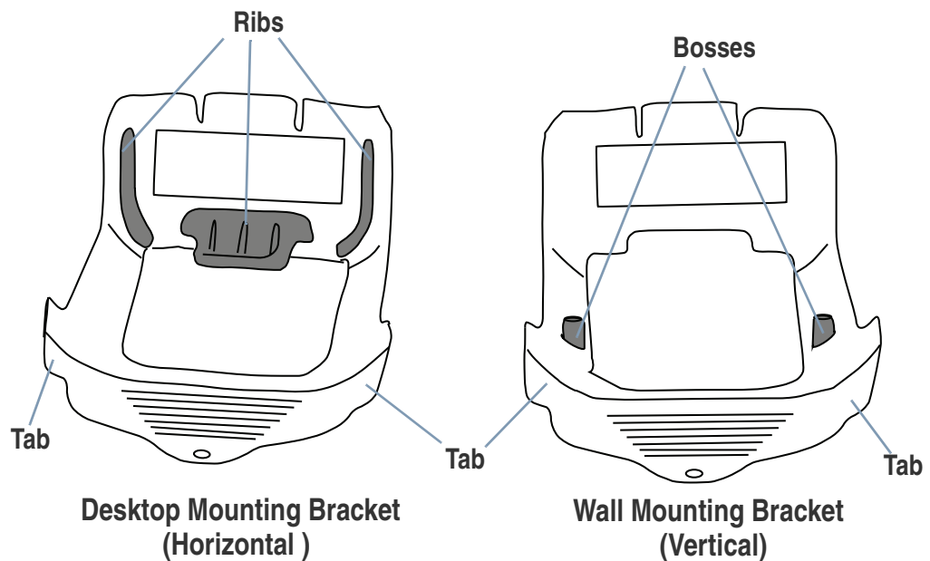
Figure 1. Mounting Brackets
